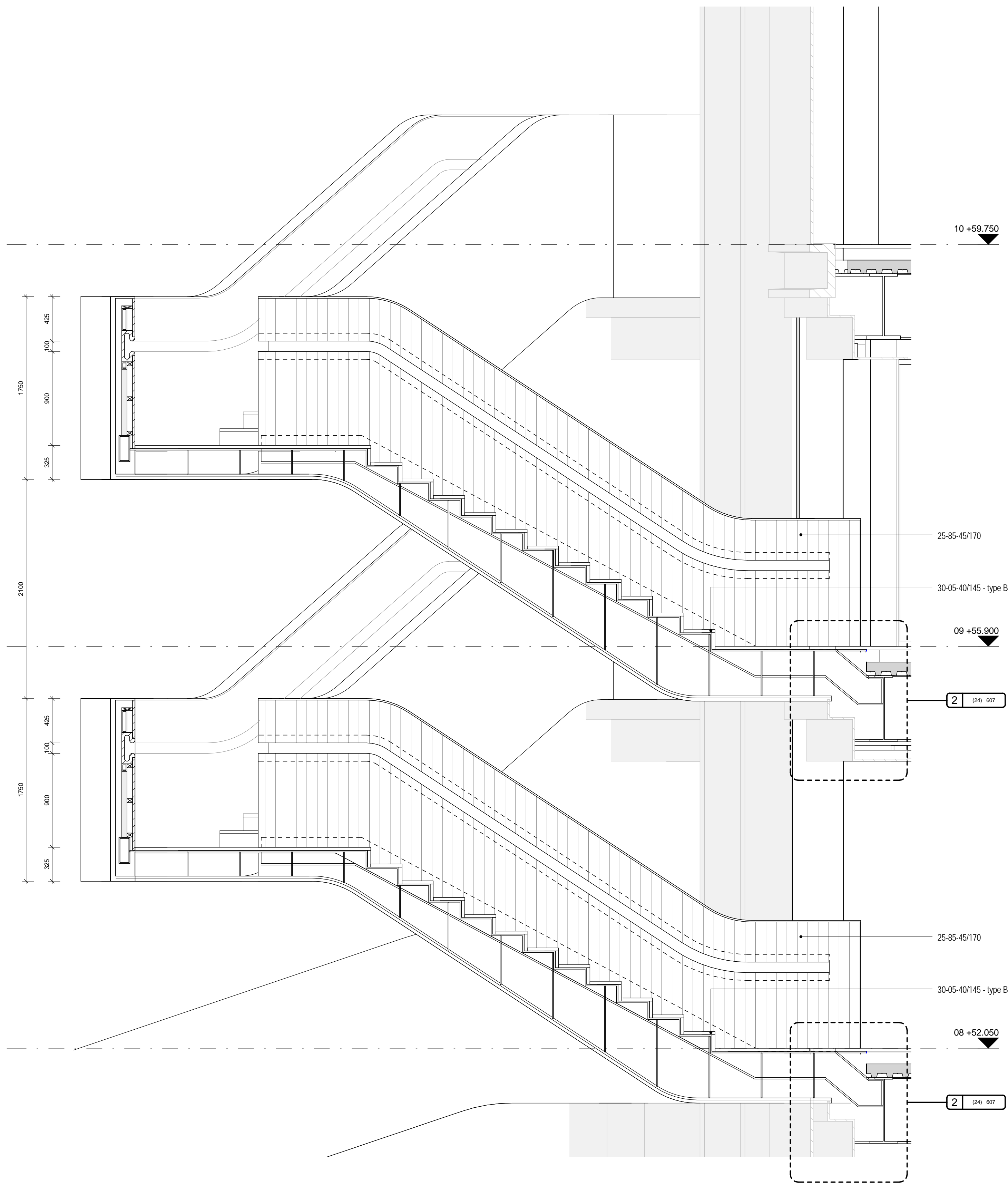
1 Stair 4 Section_1, 1 : 25@A1
