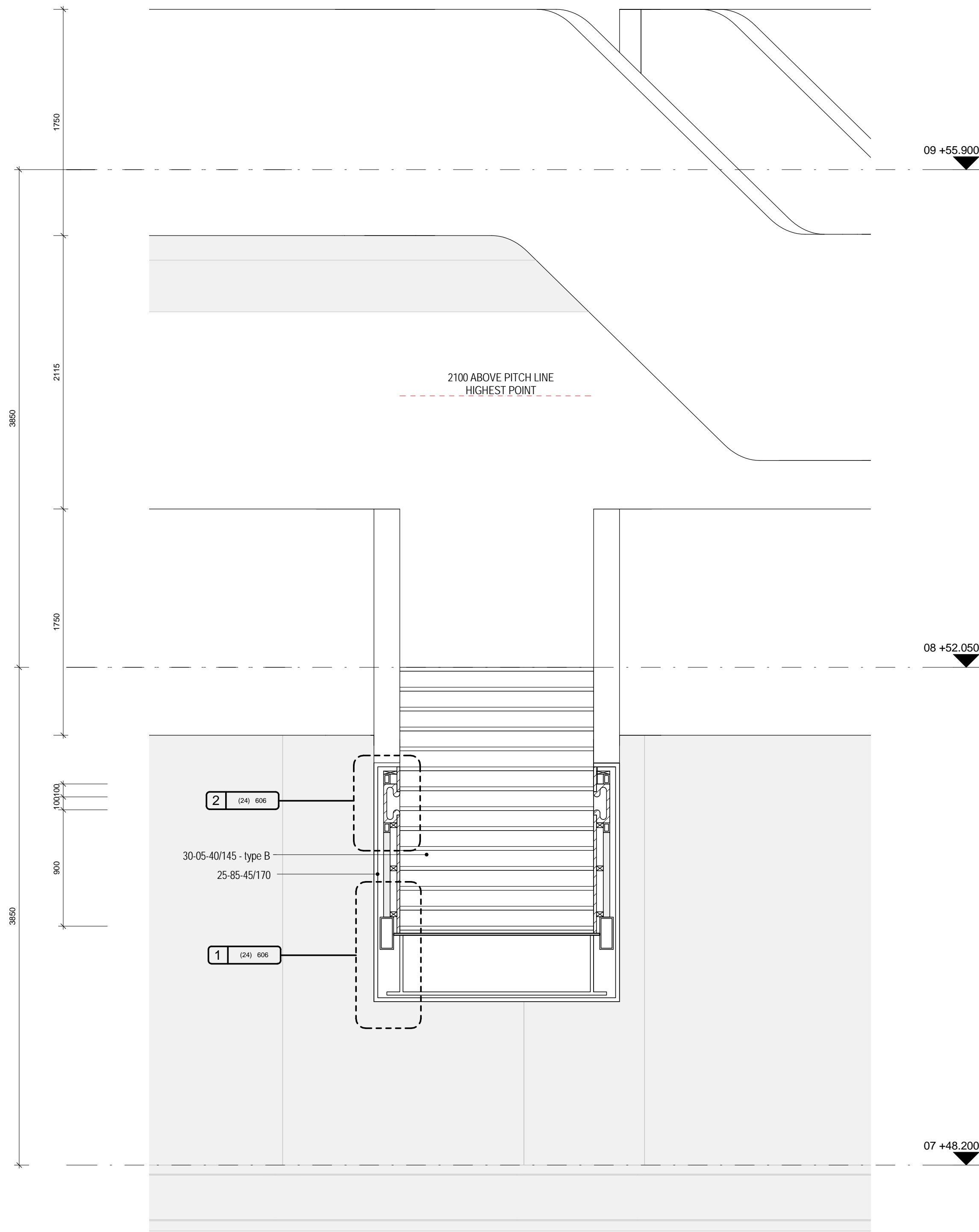
1 Stair 3 Section_1, 1 : 25@A1
