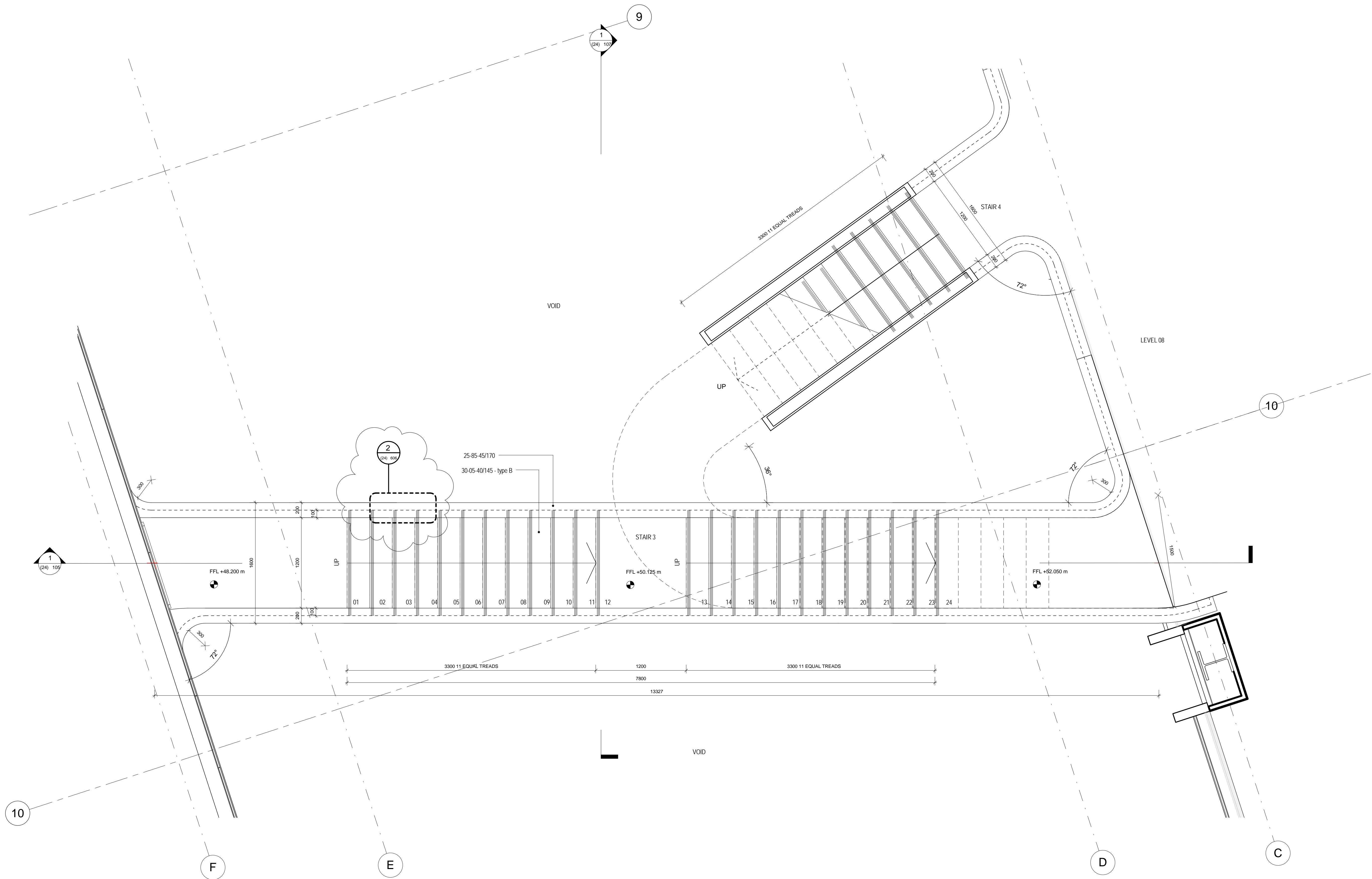
1 Stair 3 and 4 at L 08 +52.050, 1 : 25@A1
