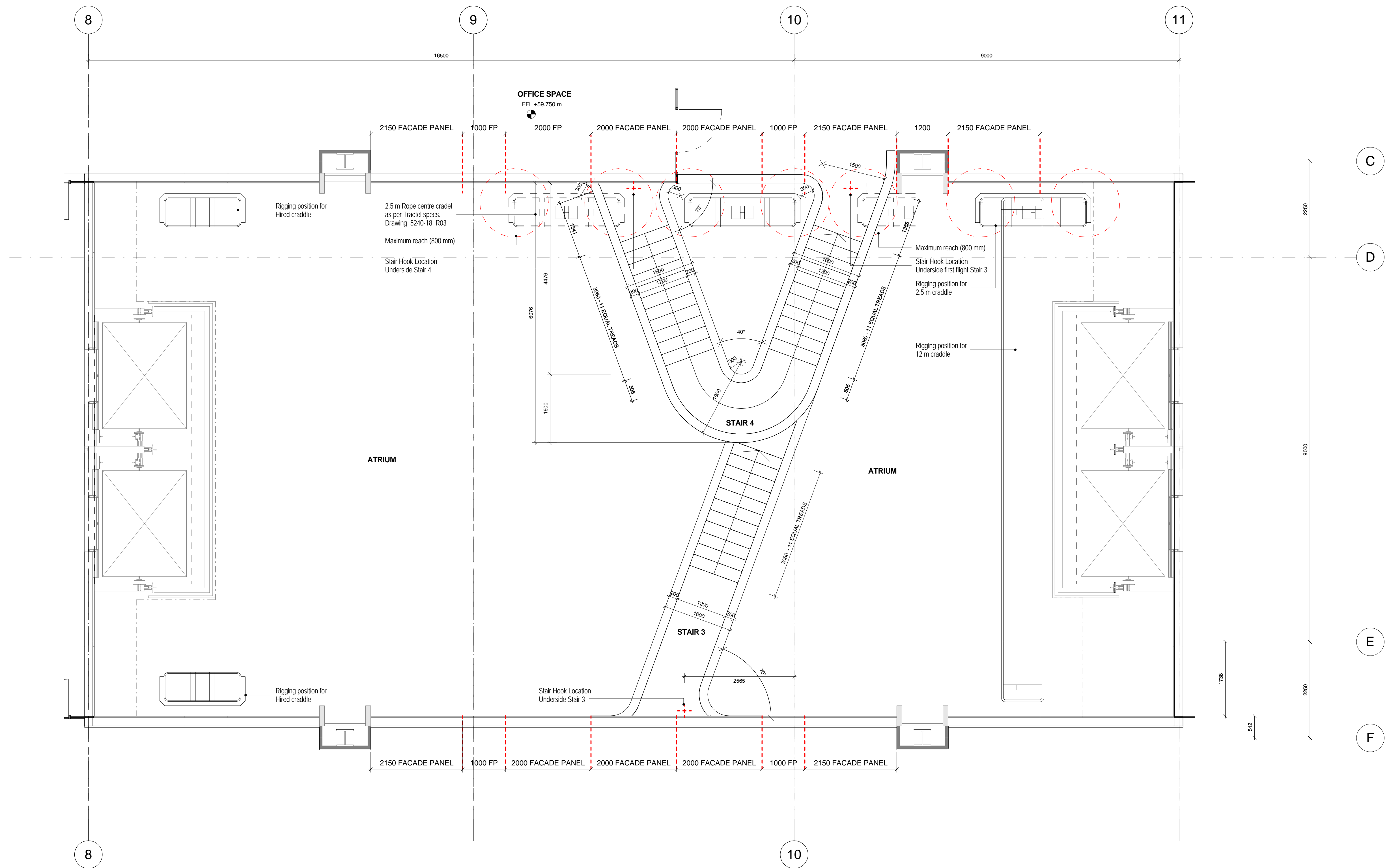
1 Atrium Stair Setout at L10, 1 : 50@A1
