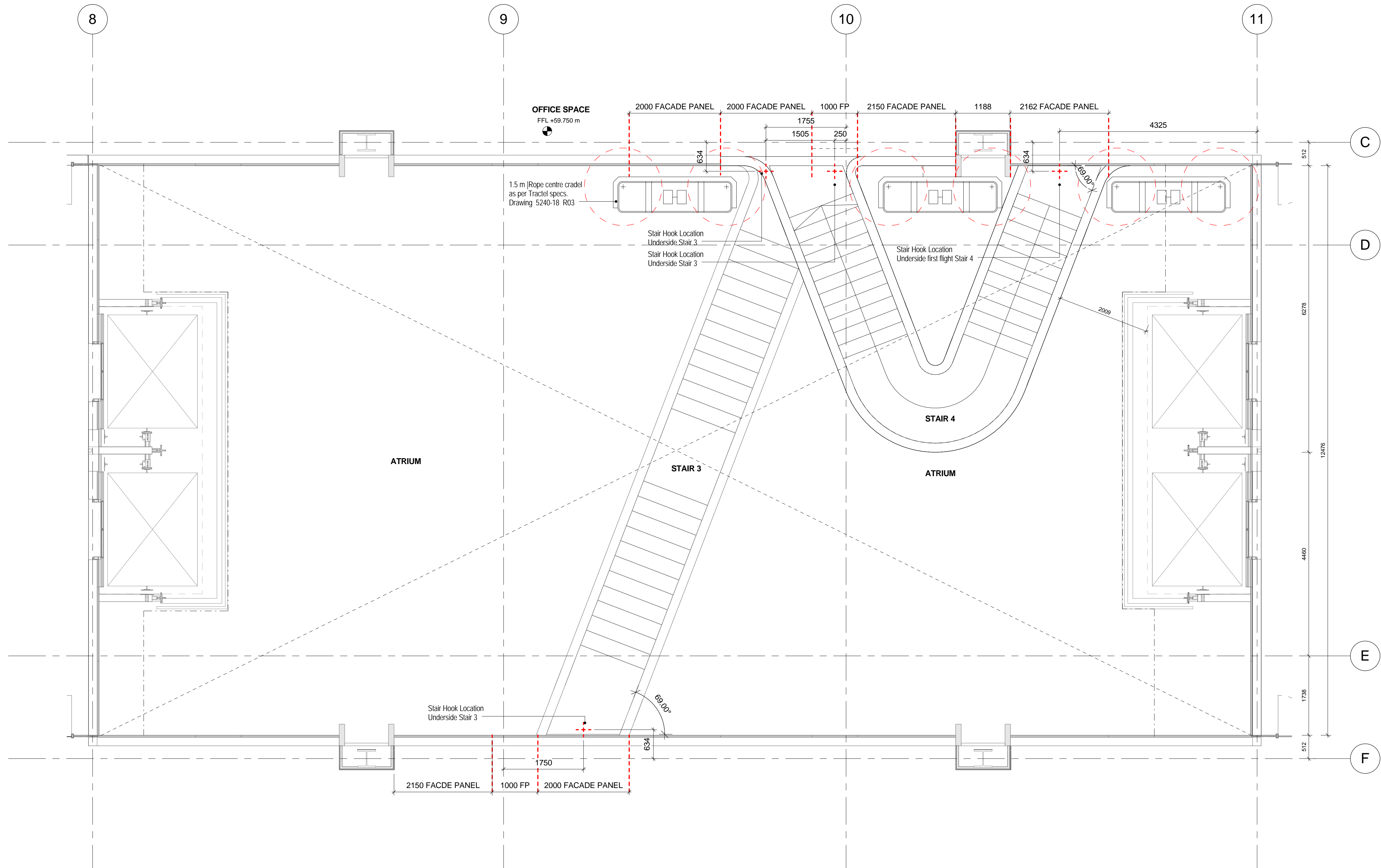
1 Atrium Stair Setout at L10, 1 : 50@A1
